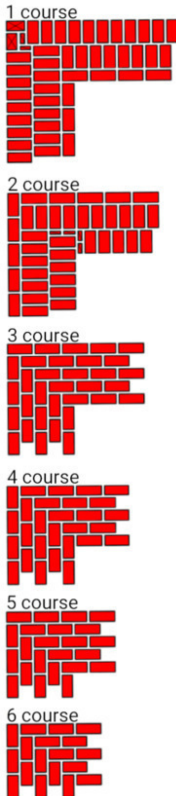
Fig.6. The order of laying bricks in the corner of the walls. Wall thickness 2.5 brick.
