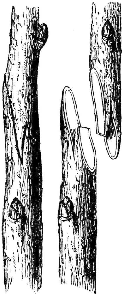
Fig. 8.—WHIP GRAFTING.
