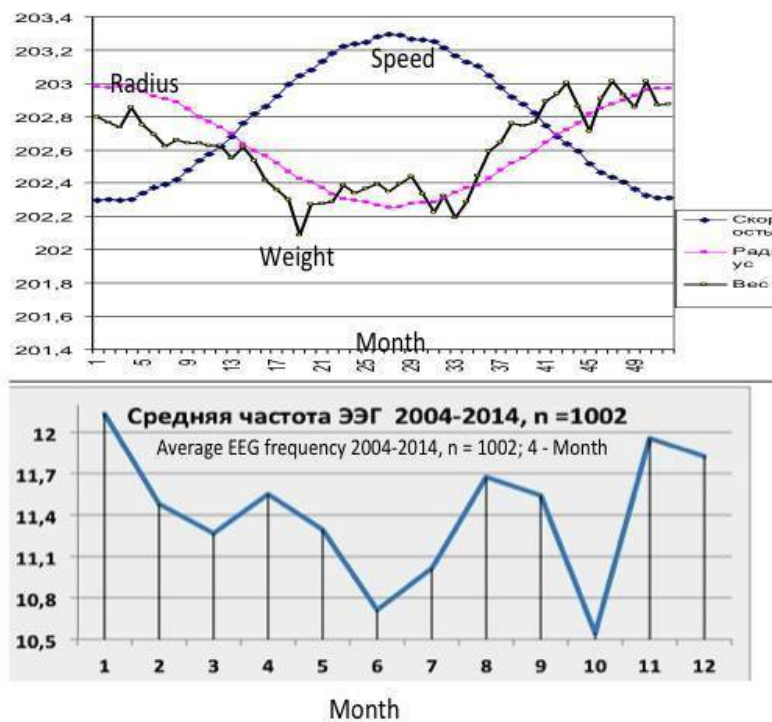
Graphs of changes of the Earth's orbital velocity and the average EEG frequency
