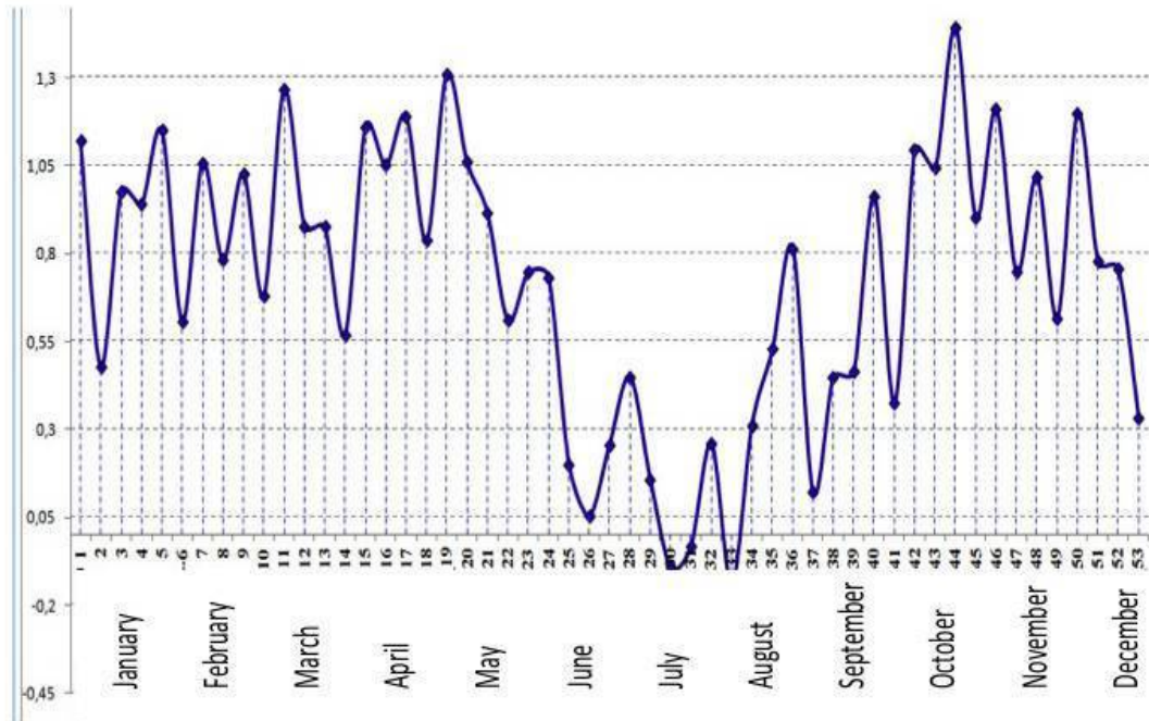
Earth LOD data 2000 in ms average by week (example)
