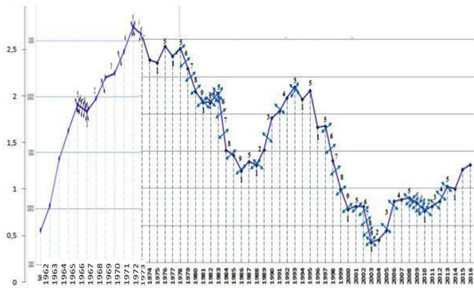
Earth LOD data since 1962 in ms
