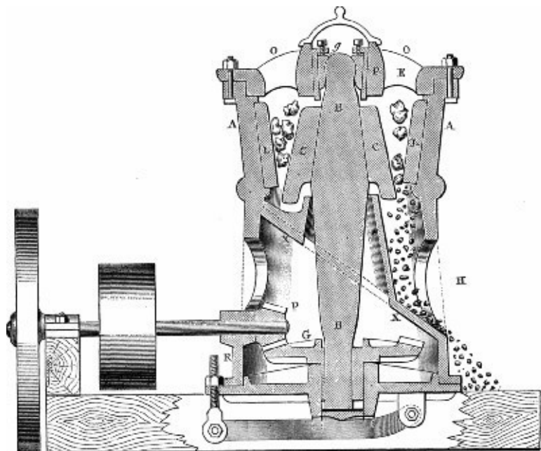
Fig. 1—BROWN'S ORE CRUSHER.
